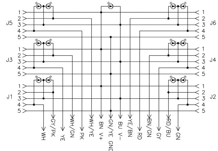
WIRING DIAGRAM
